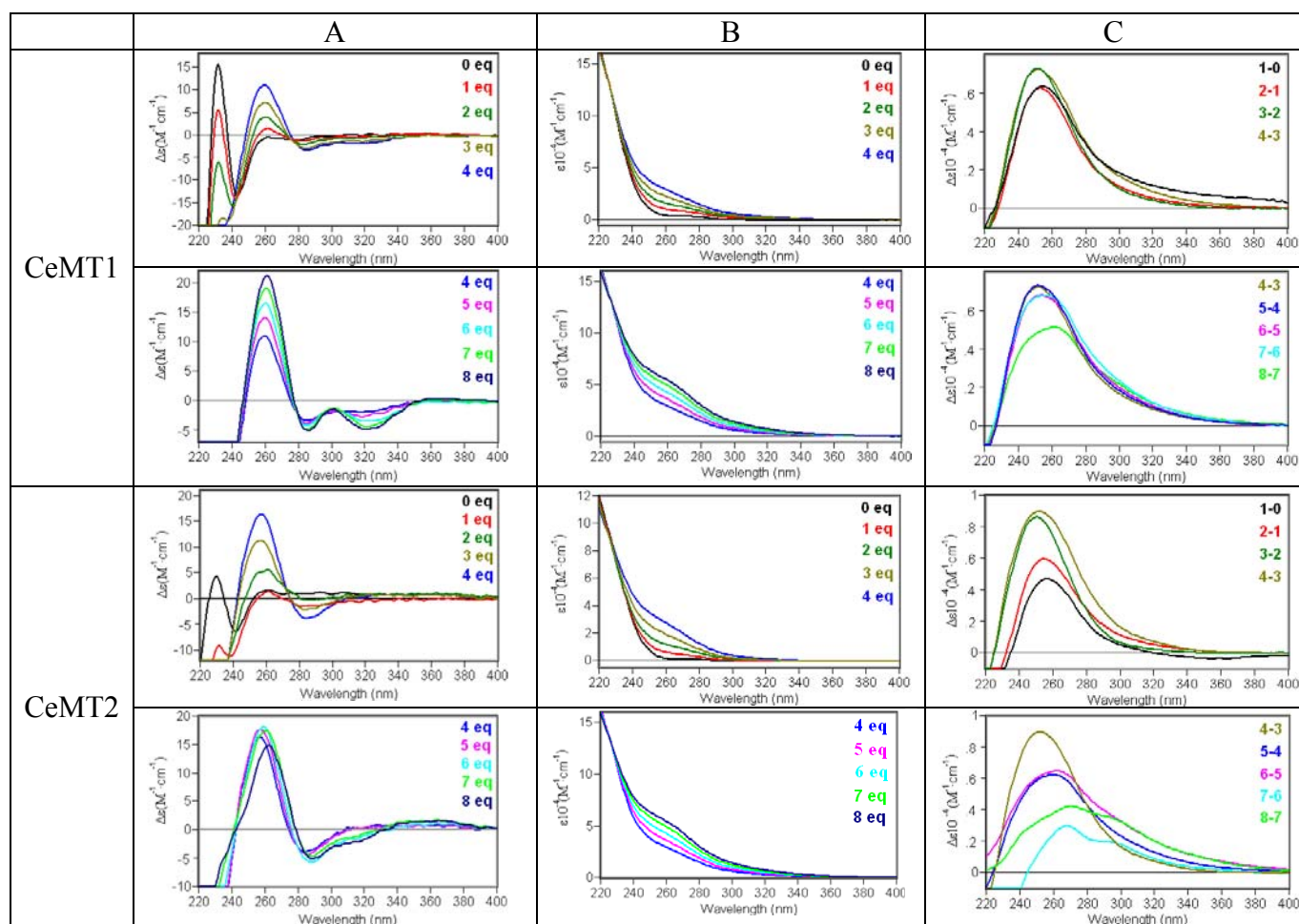
Figure 7- CD (A), UV-vis (B) and UV-Vis difference (C) spectra corresponding to the titration of a 10 \mu\text{M} solution of Zn(II)-CeMT1 and Zn(II)-CeMT2 with Cu(I) at pH 7.0.
