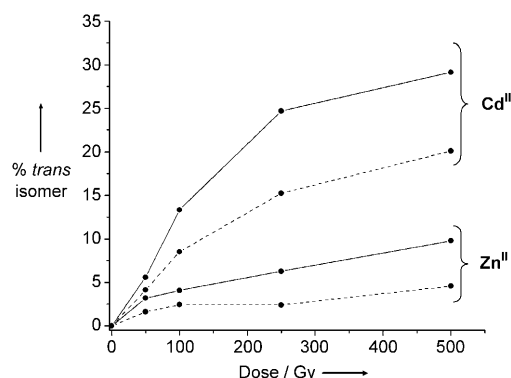
Figure 2. Dose dependence of the formation of elaidate ( trans isomer) residues from γ irradiation of POPC vesicles (2 mM) containing Zn-QsMT or Cd-QsMT aggregates (30 μM) in Ar-flushed (solid line) or N 2 O-saturated (dashed lines) 10 mM H 2 PO 4 - solutions at pH 7.
