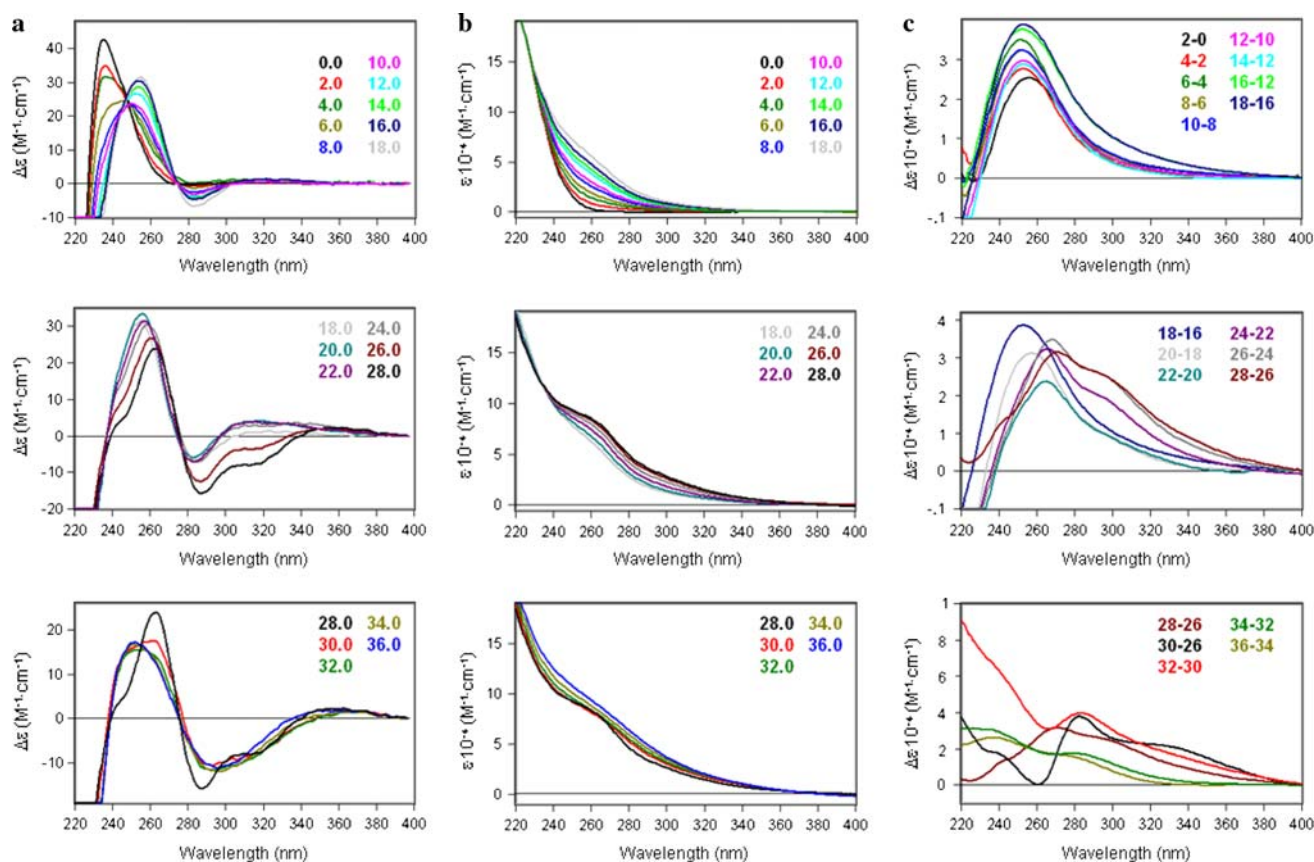
Fig. 6 a CD, b UV-vis and c UV-vis difference spectra obtained during the titration of a 10 \mu\text{M} solution of \text{Zn}_7\text{-MeMT} with \text{Cu(I)} at pH 7
